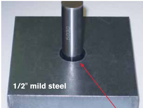
1/2" hole without True Hole technology cut with HPRXD® Plasma
